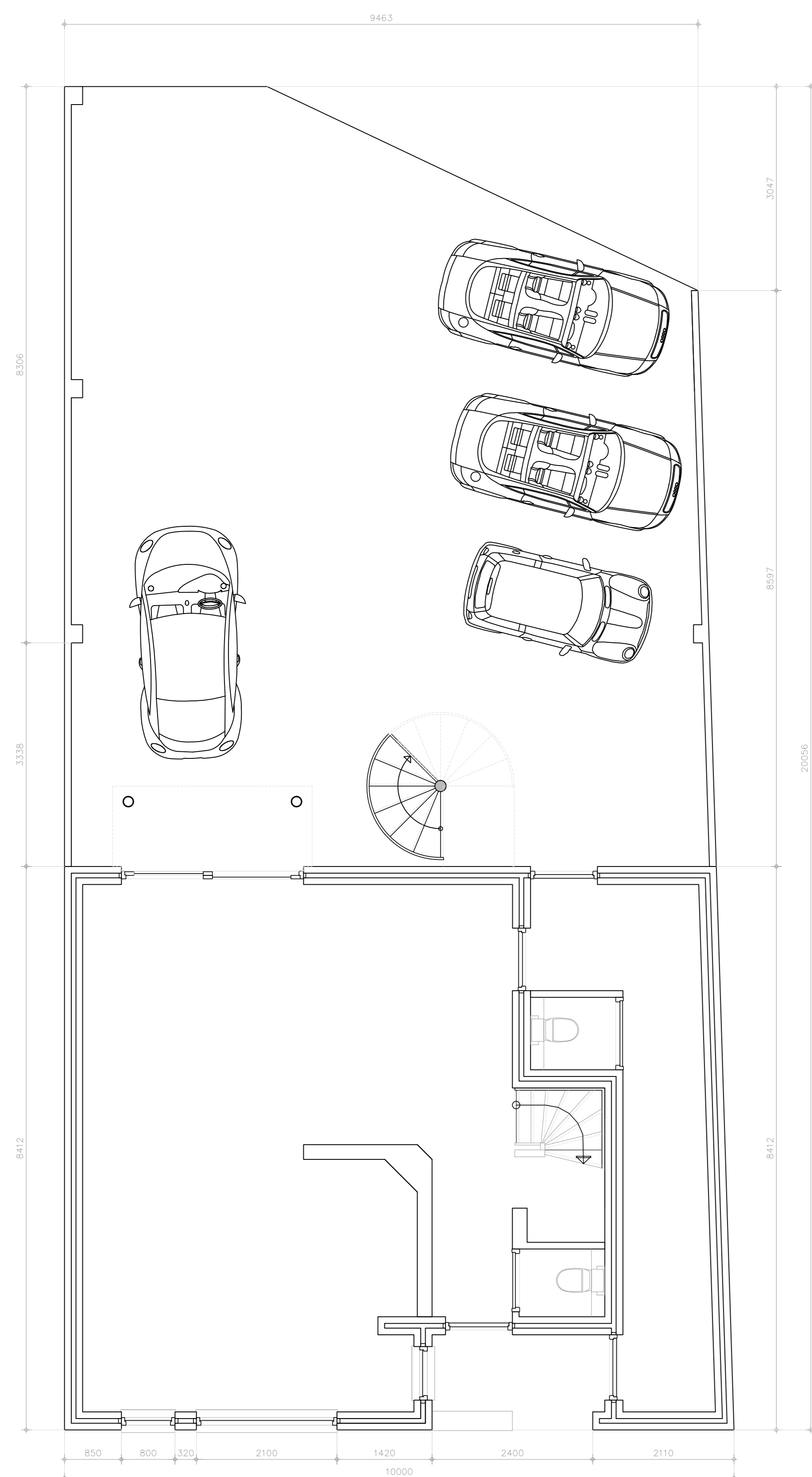
-begane grond-
